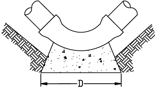
90° BEND PLAN
