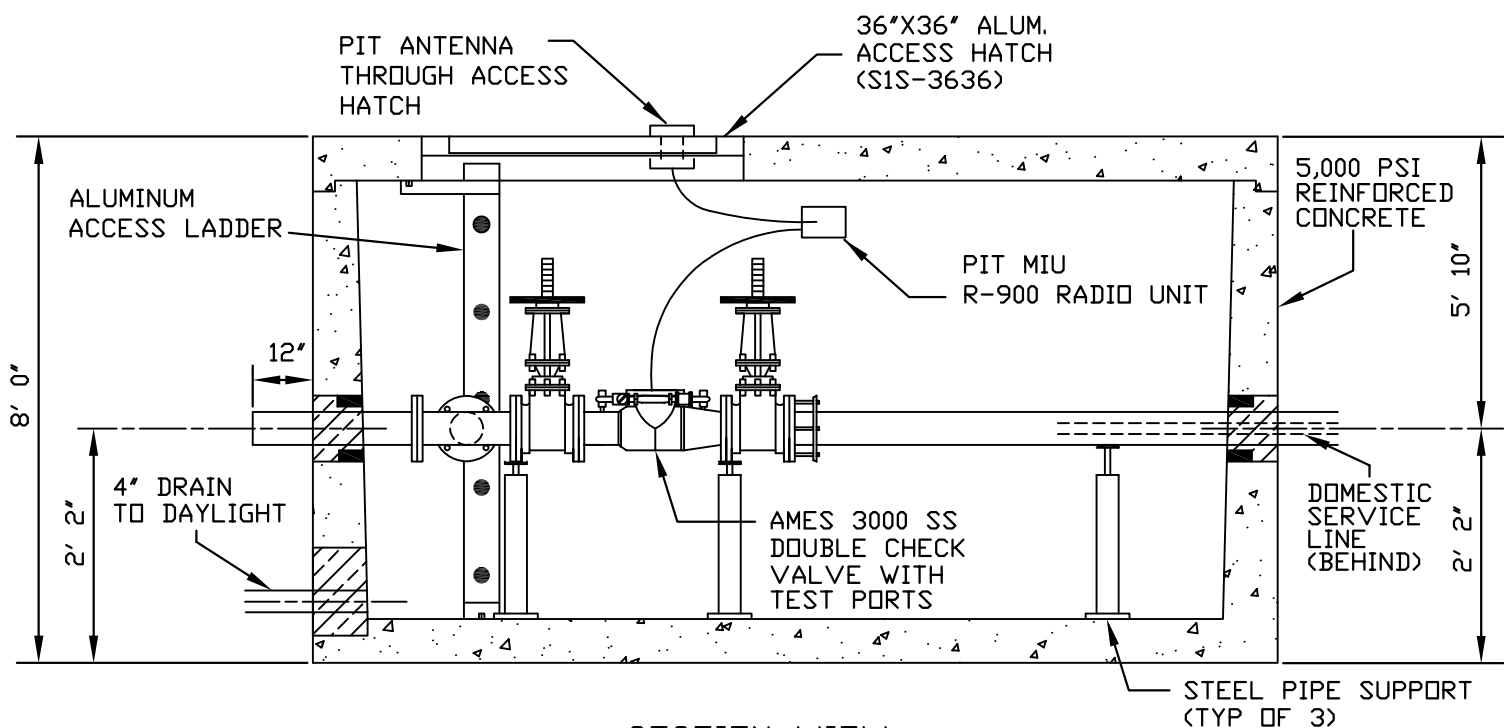
SECTION VIEW
