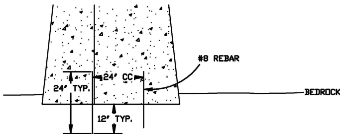
ALTERNATE "A" SIDE VIEW
